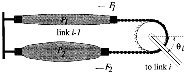
Fig. 2. An agonist and an antagonist rubeuator are connected via a chain across a sprocket; their relative lengths determine the joint position \theta_i .
