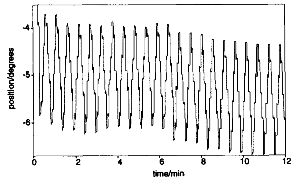
Fig. 6. Drift of the rubeatuators when the robot is used for a long period of time. The pressures of the rubeatuators are repeatedly increased/decreased by 1% of the total pressure.
