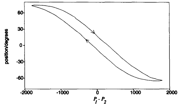
Fig. 4. Joint 1 of the robot arm as moved by applying a constant pressure increment \Delta P to rubeatuator 1 and the same decrement to rubeatuator 2. When the extreme pressures are reached, the direction is reversed.
